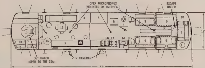
SEALAB II. Interior arrangement; Top removed-looking down. 1. Swim gear stow. 2. TV. 3. Lab bench. 4. Fan room. 5. Electric power and light. 6. Reefer. 7. Head. 8. Locker. 9. 2 Berths. 10. Stow. 11. CO 2 can. 12. Table. 13. Bench. 14. Lav. 15. Table and chairs. 16. Water heater. 17. Can stow/g. 18. Tub and shower.
